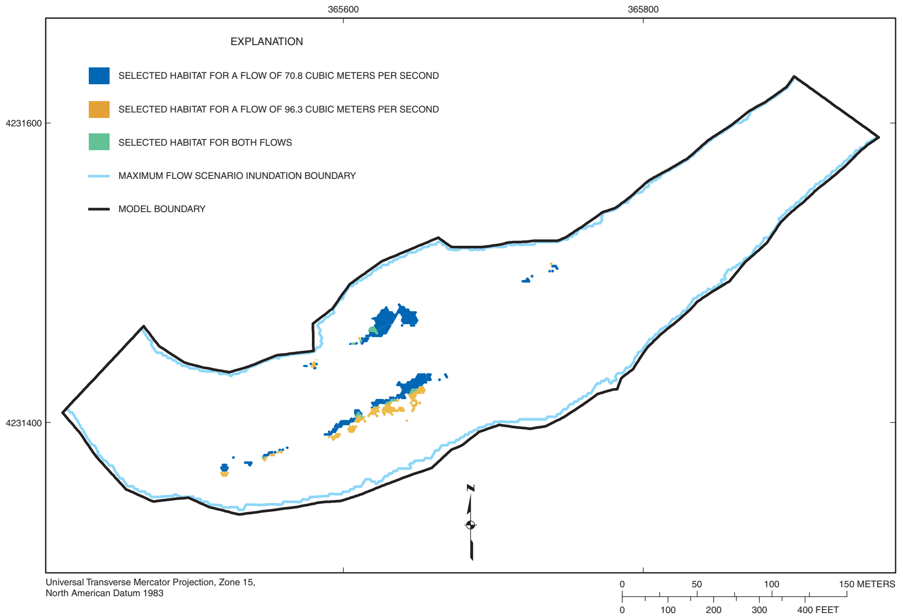
Figure 4-66. Selected habitat area distribution for habitat categories 16, 17 combined (channel catfish) at flows of 70.8 and 96.3 cubic meters per second at Marais des Cygnes River site MDC2.
